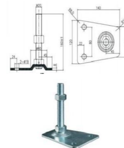
⑨杯脚
